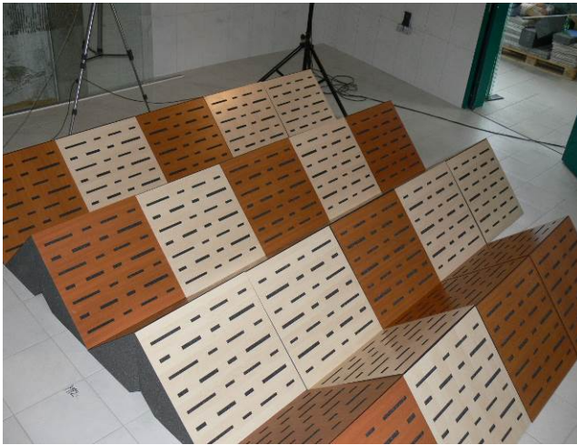
Picture 5: test samples in the reverberation room.
