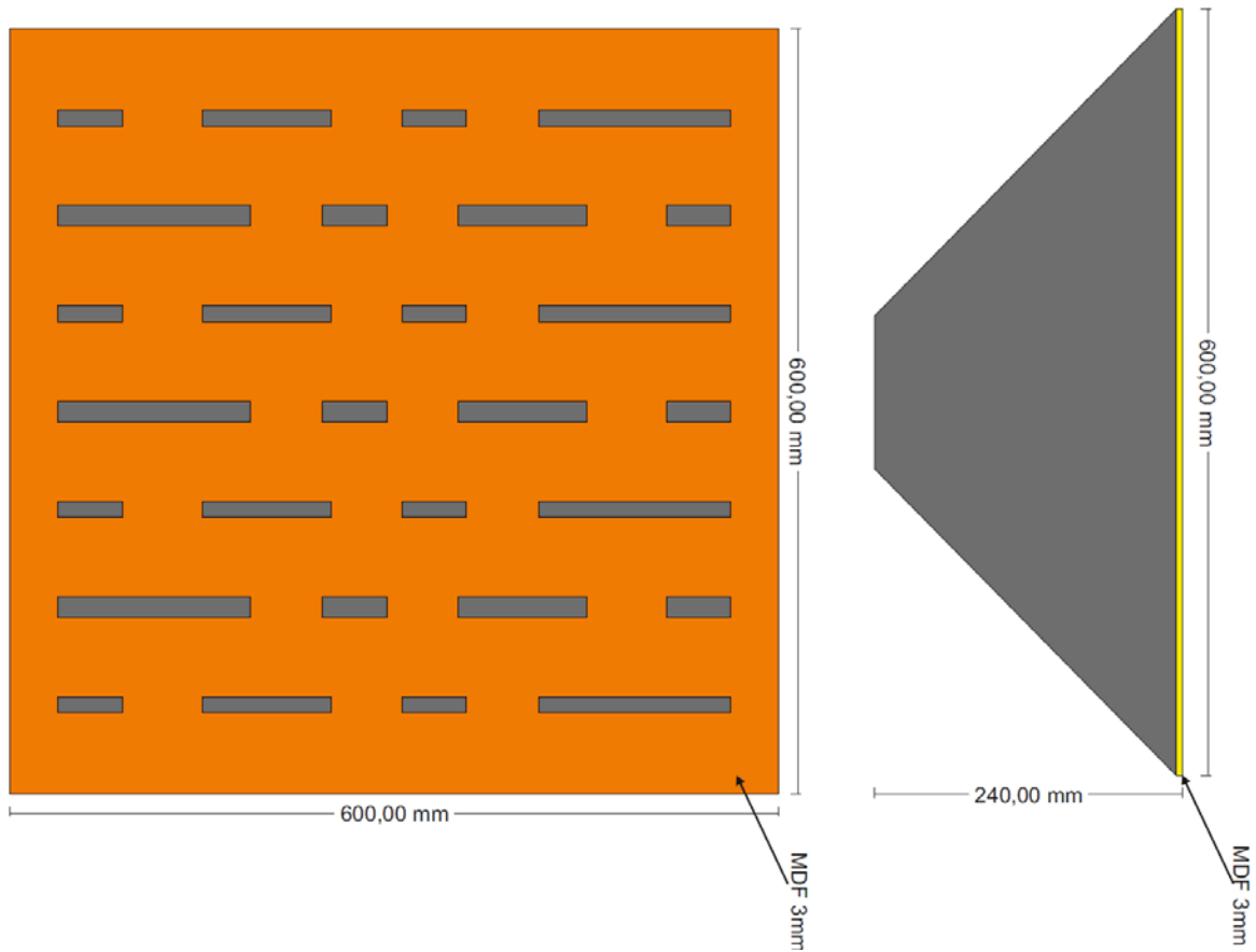
Picture 1: schematic drawing of the Decotrap sound-absorption cladding.
